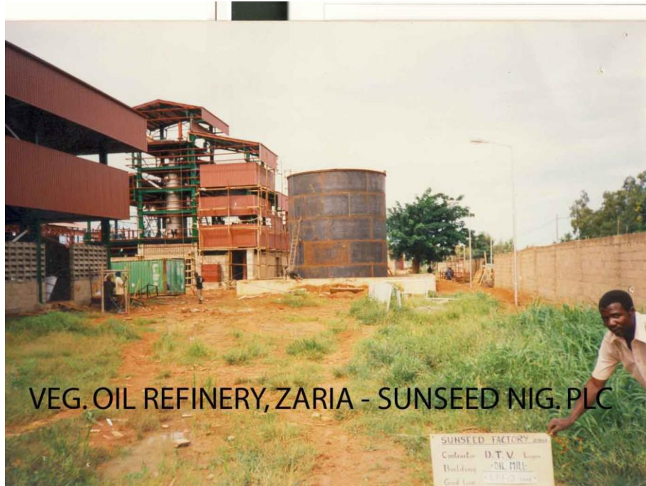
VEGETABLE OIL REFINERY, FOR SUNSEED NIG. PLC. AT ZARIA, KADUNA STATE.
